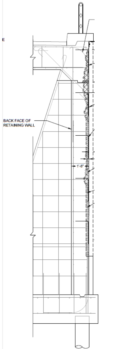
DETAIL 1 (PROPOSED) SCALE: 1/4"=1'-0"
